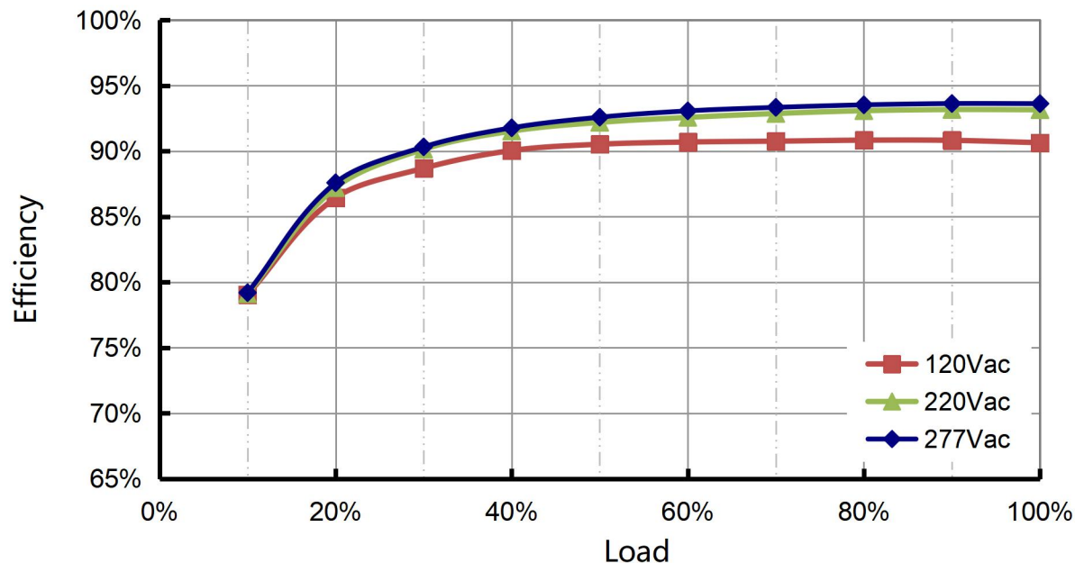
Efficiency vs. Load (V024)
